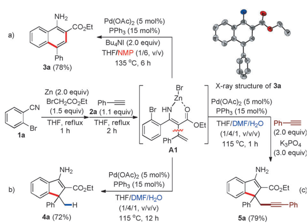
Scheme 2. Pd/solvent-controlled selective tandem synthesis of 1-aminonaphthalene 3a and indenes 4a and 5a from a common nitrile 1a .
